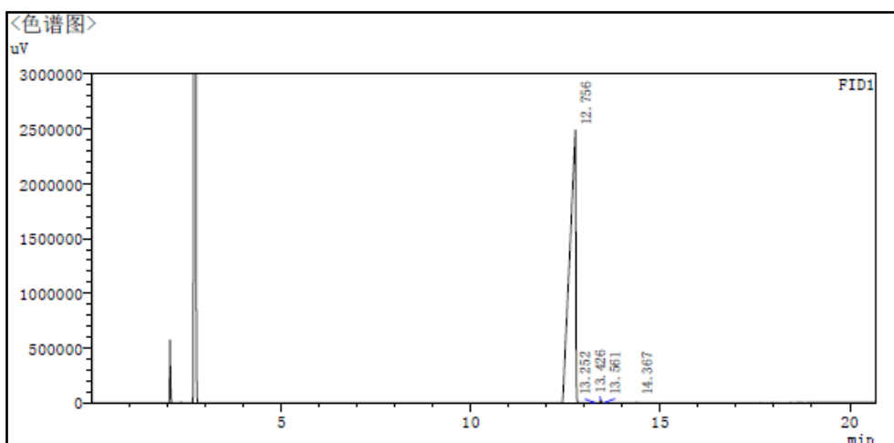
Fig.2-1 “201811050105-1”GC chromatography
